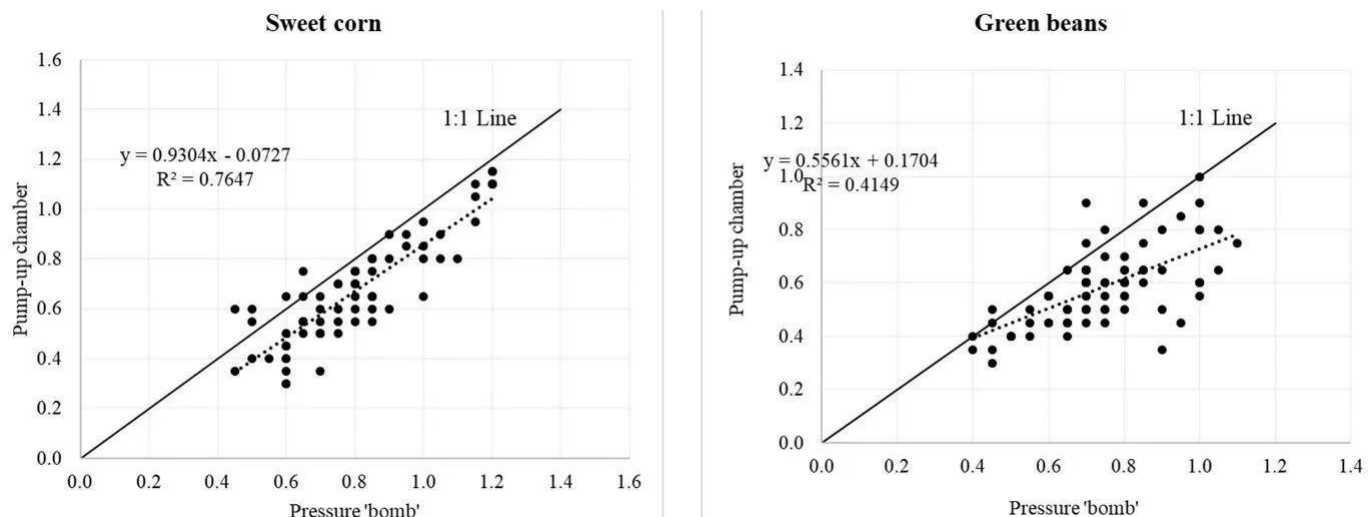
Figure 6. Comparison of leaf water potential measurements (Megapascal; Mpa) using the pressure “bomb” and pump-up chamber methods.
