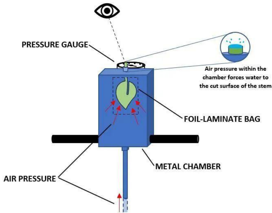
Figure 2. Schematic of a pump-up chamber. Credit: Christian Bartell, UF/IFAS
