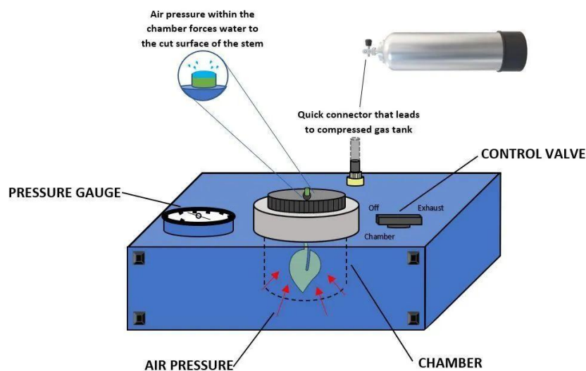
Figure 1. Schematic of a pressure "bomb." Credit: Christian Bartell, UF/IFAS
