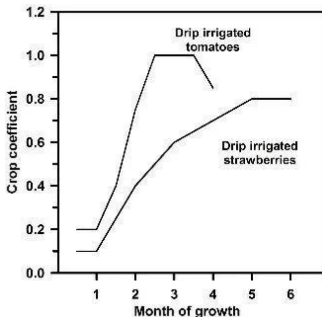
Figure 4. Crop coefficient of drip-irrigated tomato and strawberry.
