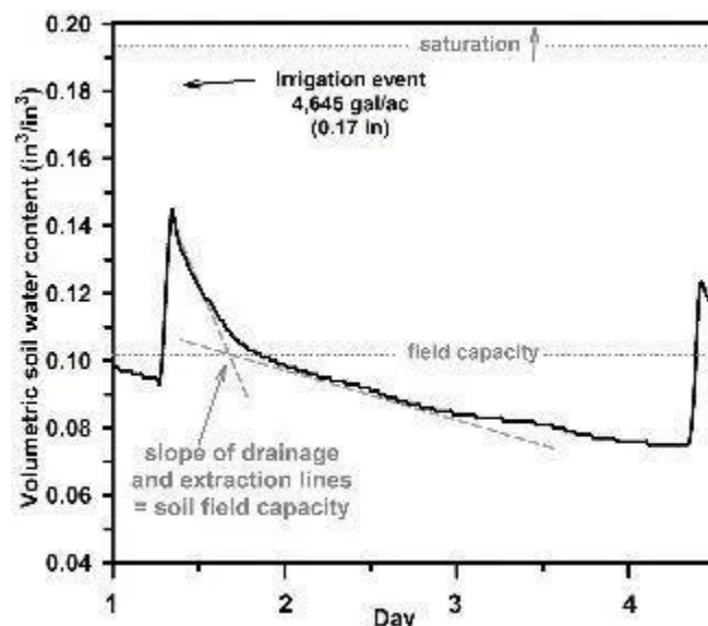
Figure 1. Example of practical determination of soil field capacity at 0–6 in. soil depth after an irrigation event using soil moisture sensors.
