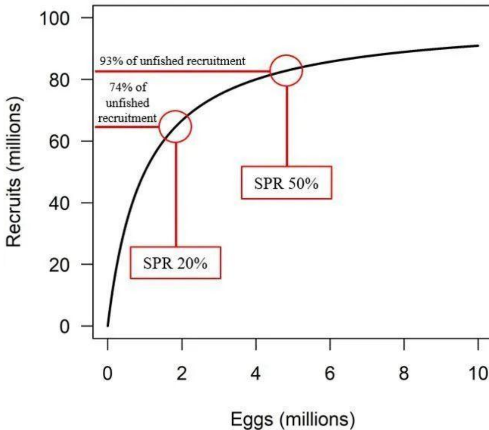
Figure 2. Example of the number of recruits (young fish) produced at two different SPR levels. Credit: UF/IFAS
