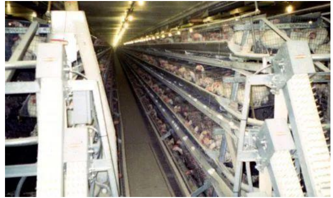
Figure 5. An example of a caged-layer poultry cage. Credit: Phillip E. Kaufman, UF/IFAS
