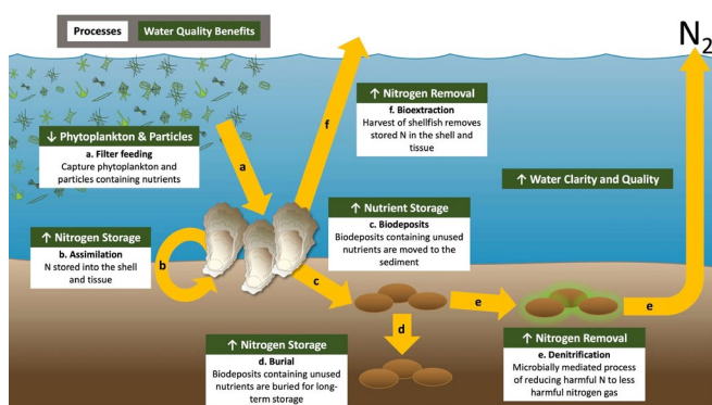
Figure 1. Ecological processes and water-quality benefits associated with oysters improve water clarity and provide nitrogen removal.
