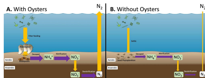
Figure 2. Sediment nitrogen cycling processes (A) with oysters and (B) without oysters.
