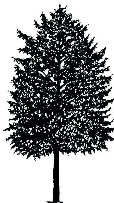
Figure 1. Middle-aged Acer platanoides 'Cleveland': 'Cleveland' Norway Maple
