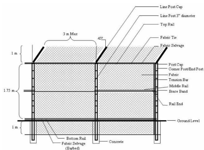
Figure 8. Fence design for a crocodilian enclosure located upon solid ground with inward facing 45° turn at the top.
